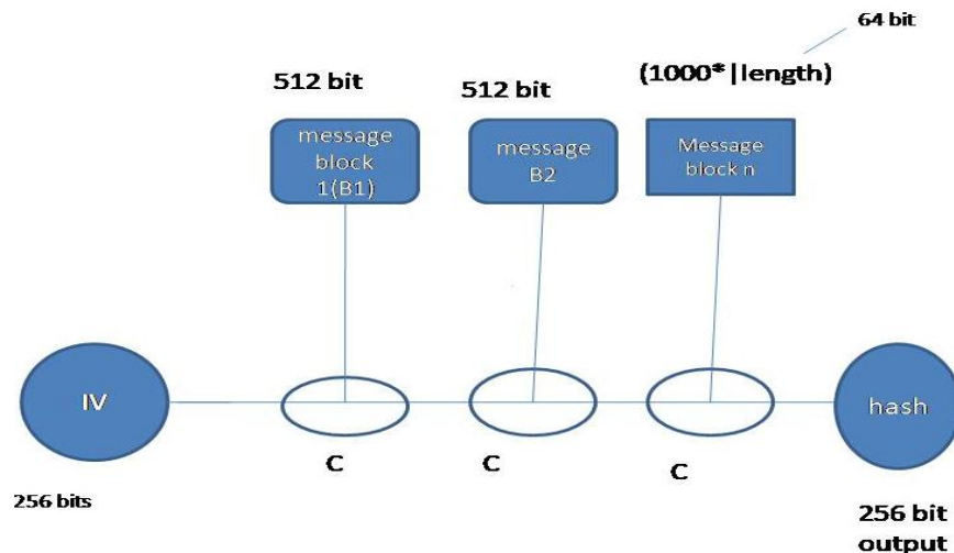
Figure 1. Prototype of Algorithm
